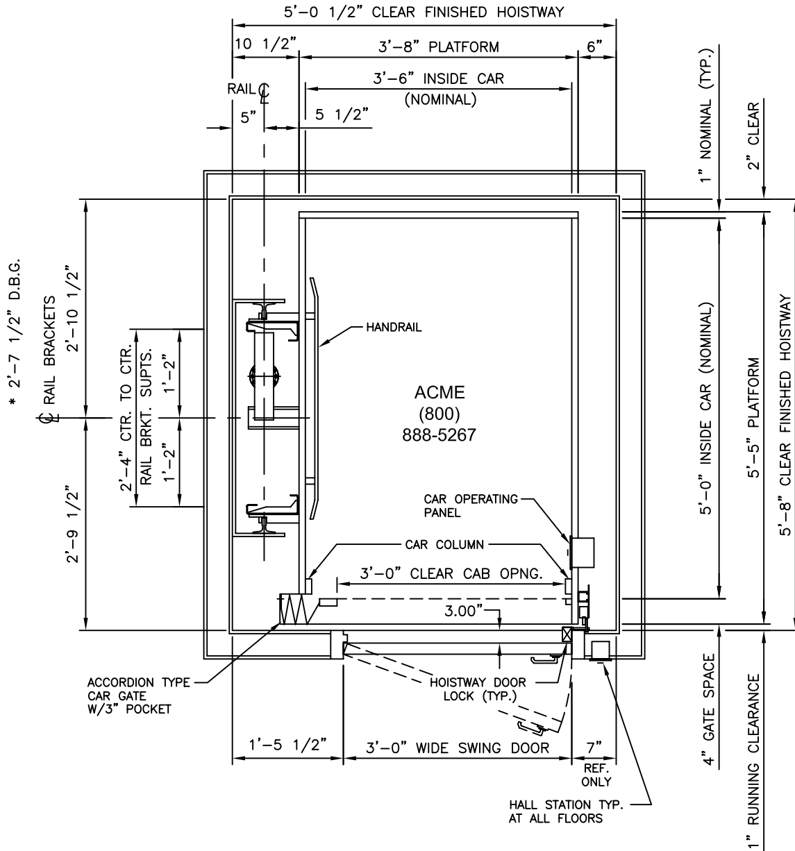
TYPICAL 1400-18 FLOOR PLAN SWING DOOR
